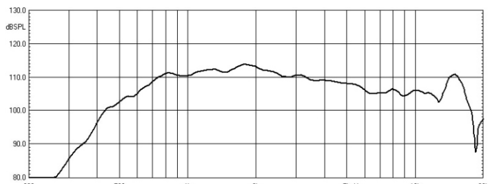
Frequency response curve of the driver measured with 1w input on rated impedance at 1m distance on axis from the mouth of horn.
